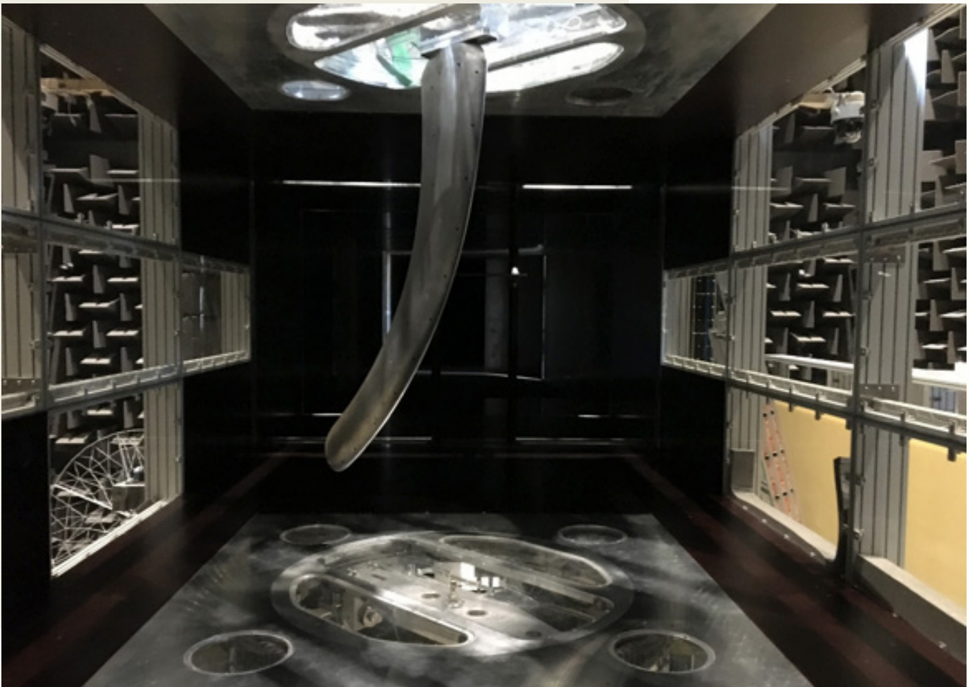
Figure 1. Swept blade tip measured in a DTU-PLC wind tunnel.
