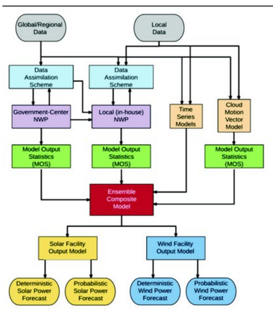
Figure: High-level overview of the components and data flow of a typical state-of-the-art forecasting solution.
