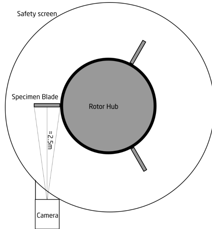
Figure 10 Illustration to approximate scale of the average R&D A/S RET, with camera position shown and approximate distance from camera to specimen at imaging position.
