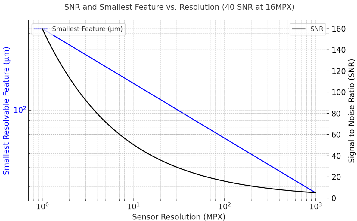
Figure 6 Effect of Increasing Sensor Resolution on SNR.
