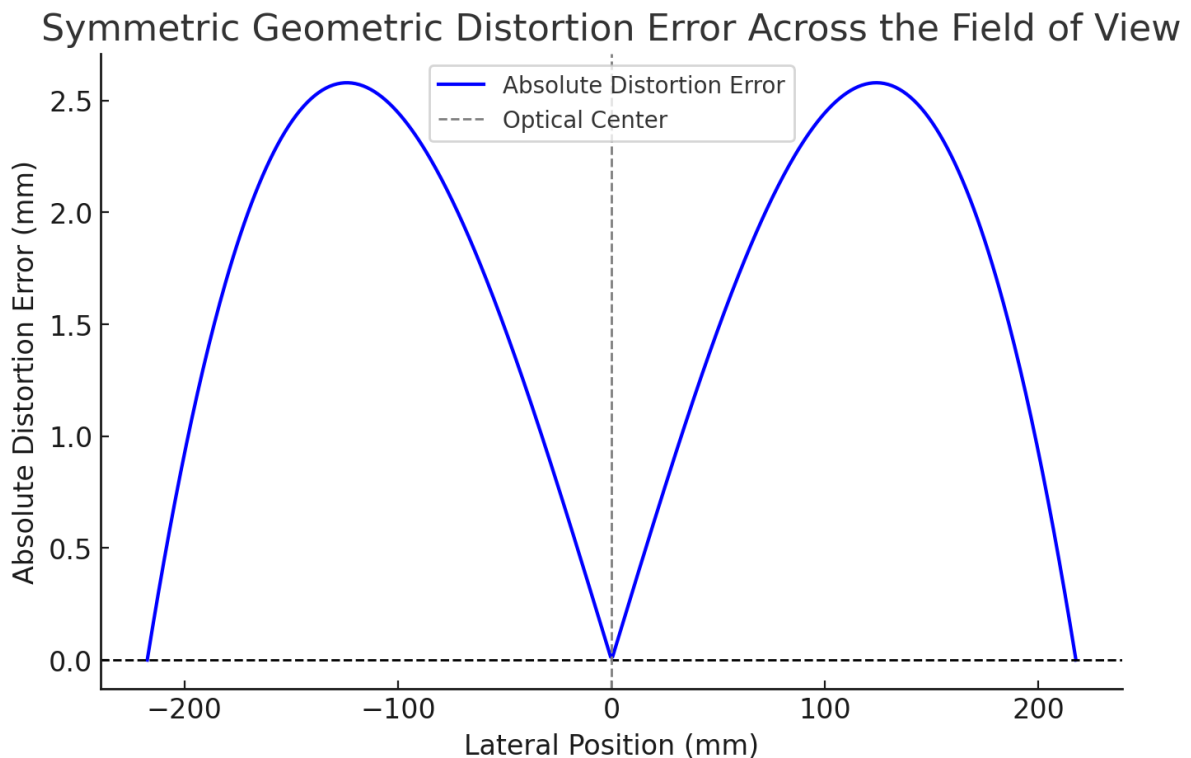
Figure 15 M-shaped absolute error in measured distance relative to the optical center, with known positions at both ends of the sample.
