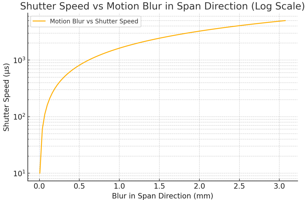
Figure 11 Relationship Between Shutter Speed and Motion Blur.
