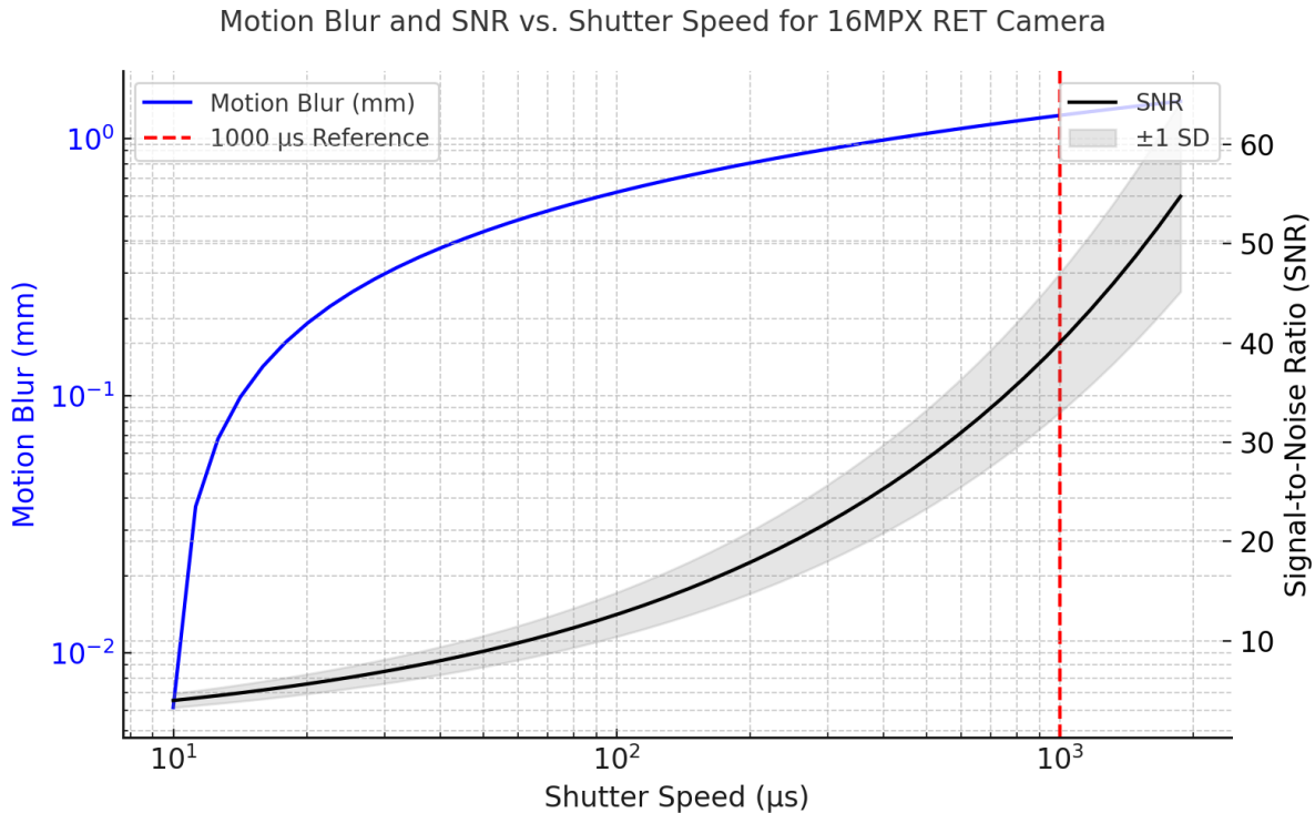
Figure 13 Motion Blur and SNR vs. Shutter Speed for the 16MPX RET Camera.
