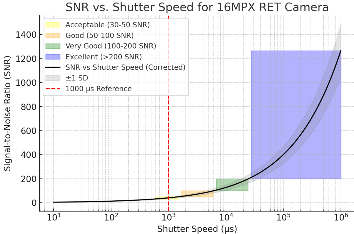
Figure 12 SNR vs. shutter speed for the 16MPX RET camera, showing how signal-to-noise ratio decreases as exposure time is reduced. The shaded regions indicate different quality levels for analytical work, with a red dashed line at 1000 μs marking the reference SNR of 40.
